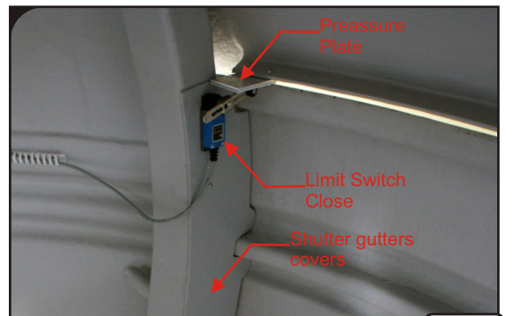
Limit switch CLOSE
