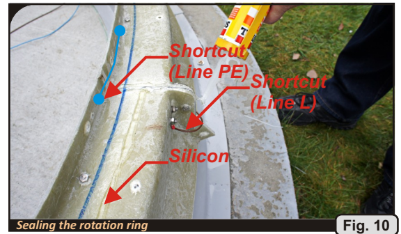
Sealing the rotation ring
