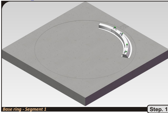
Base ring - Segment 1
