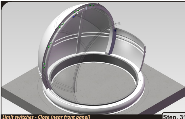
Limit switches - Close (near front panel)
