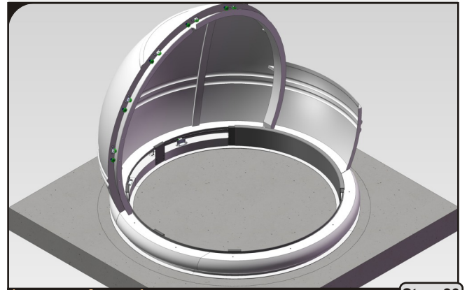
Inner covers - Segment 1
