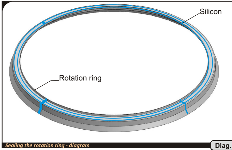
Sealing the rotation ring - diagram
