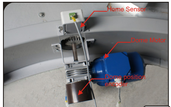
Rotation drive module mounted on the base ring
