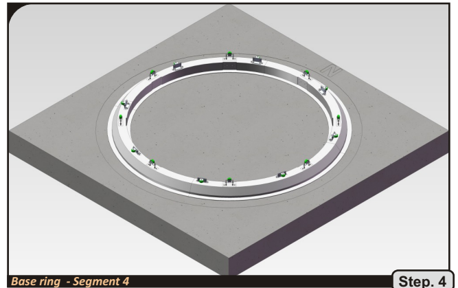
Base ring - Segment 4
