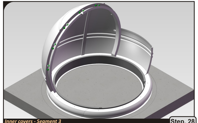
Inner covers - Segment 3
