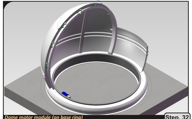
Dome motor module (on base ring)
