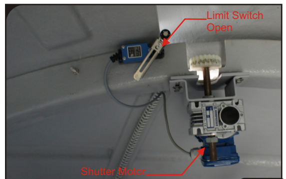
Limit switch OPEN
