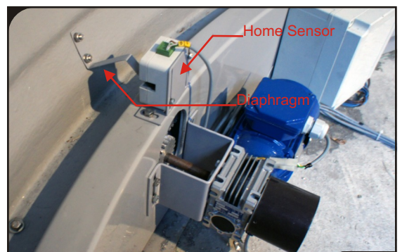
Home Sensor and its diaphragm
