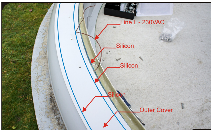
Outer cover ring sealing scheme
