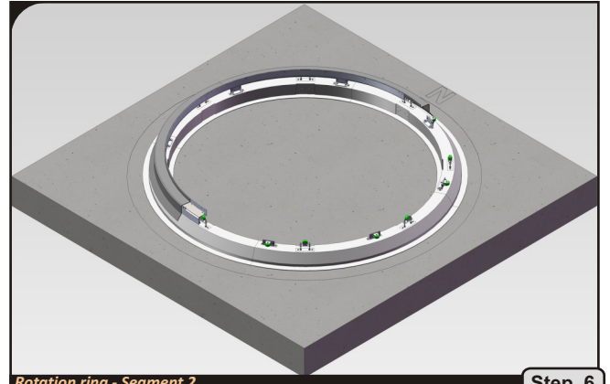
Rotation ring - Segment 2
